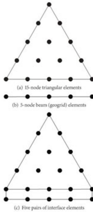
FIGURE 4: Basic elements used in the numerical model.
